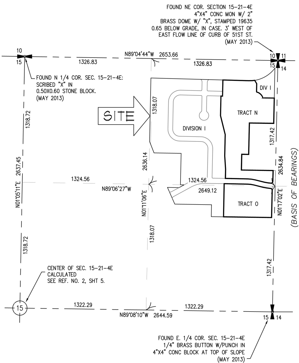
SECTION AND PARCEL DETAIL
